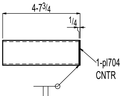
ONE HSS F-13.03M1
