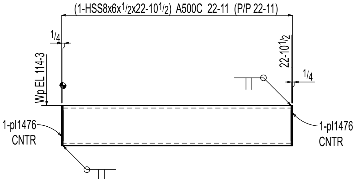
ONE BEAM F-13.03B2
