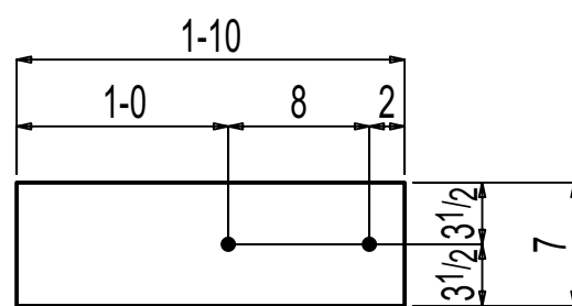
ONE PLATE F-13.03P2
