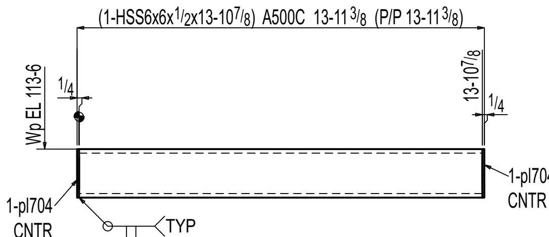
ONE BEAM F-13.03B3
